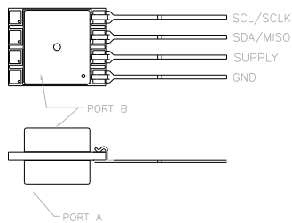
VERTICAL HOLE, DUAL, S/SL PIN STYLE
