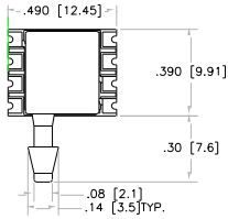
HORIZONTAL BARB, TOP
